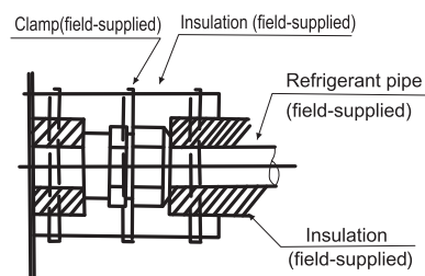
Piping insulation procedure
