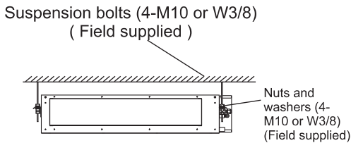
Fig. 3.4 The installation of the indoor unit
