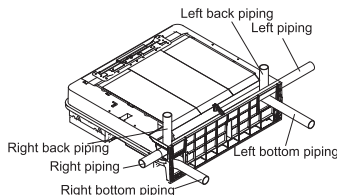
Fig. 4.1 The connection positions of the tube
