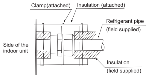
Fig. 4.4 Piping insulation procedure
