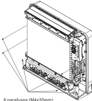
6 parafusos (M4x30mm)
