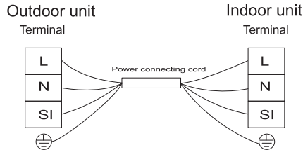
Electrical wiring diagram
